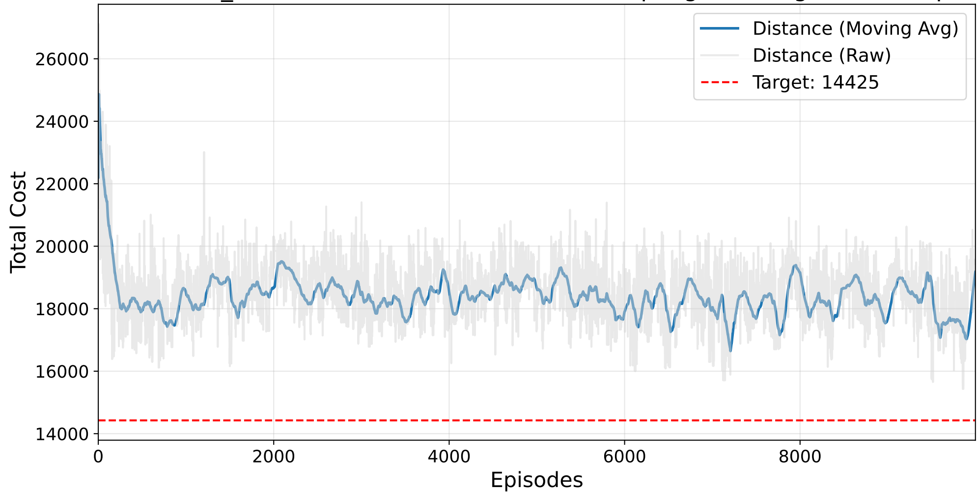
Final NO_MASK Masked AutoRL-SOP (Resampling) Training - ft53.4.sop
